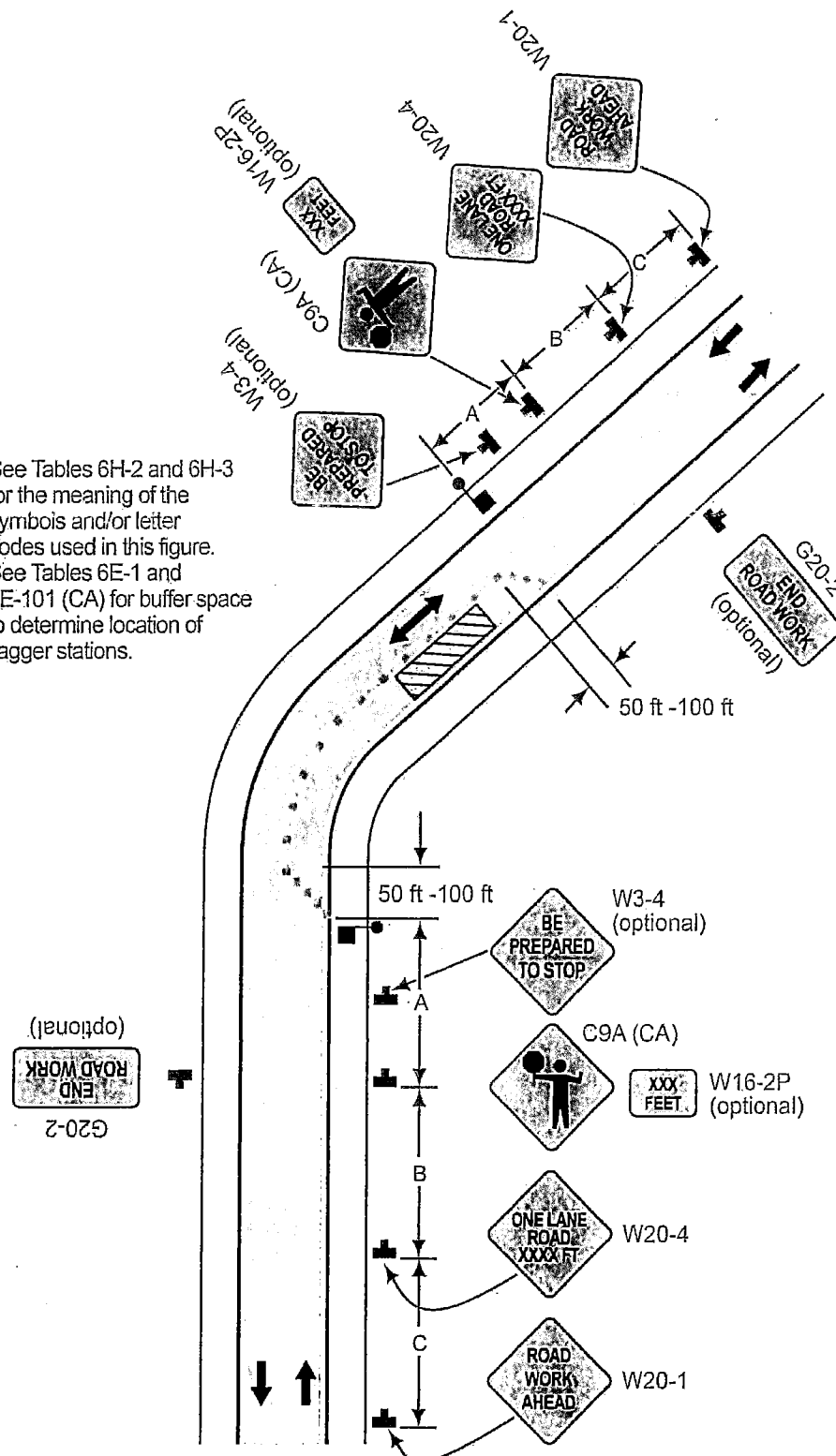
Typical Application 10
